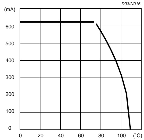
Figure 7: Max. Output Current vs. Ambient Temperature (SO20 Package, R_{th\ j-amb} = 90^{\circ}\text{C/W} )
